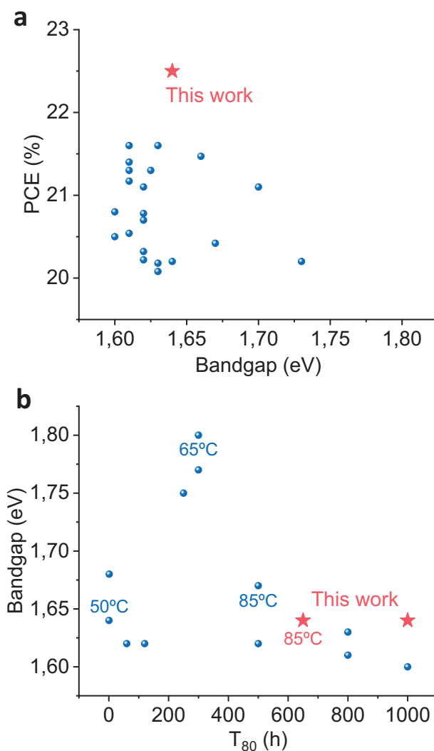
Figure 1. Device results of this work as red stars in the context of literature. a) PCEs over 20% of PSCs with an absorber bandgap of 1.6–1.8 eV. b) T_{80} of PSCs with an absorber bandgap of 1.6–1.8 eV during MPPT using ISOS protocol. Unless specified, the measurements were carried out at 20–25 °C.
